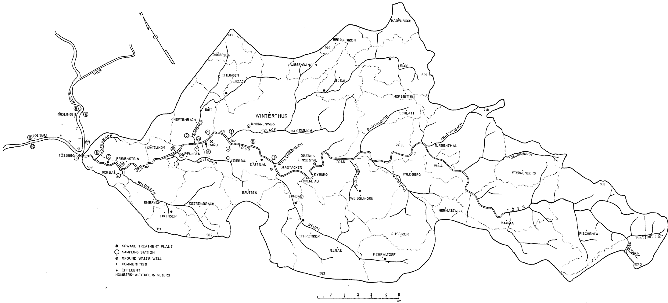
Fig. 1. Topographical Map of the River Töss Basin Showing the Sampling Stations and Principal Sources of Pollution.
